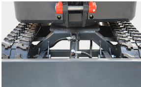
6 Thickened and widened bulldozer blade It expands the operation coverage, enables quick completion of trimming, reduces the equipment's moving path, saves operation time, is less prone to deformation or breakage and extends the service life.
